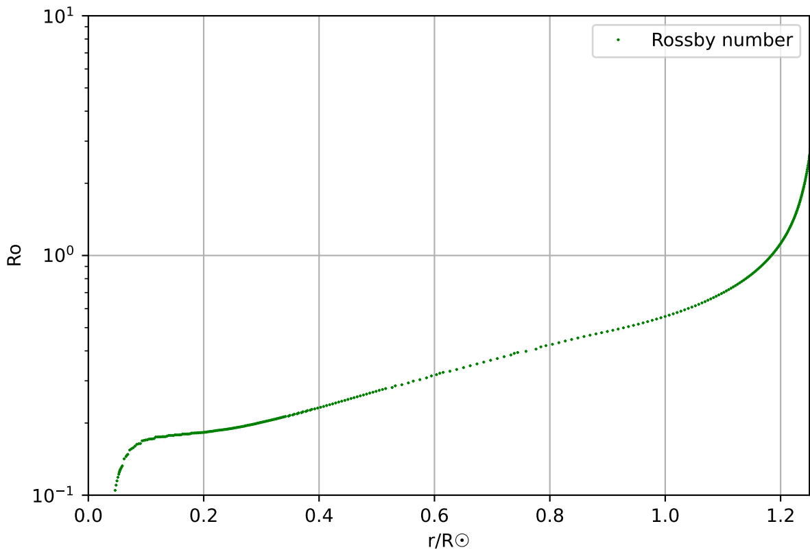
Rossby number, profile 167, age 9.65 \times 10^9
